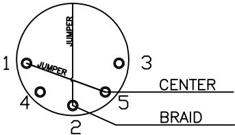
DIN PLUG Front (Mating) View
